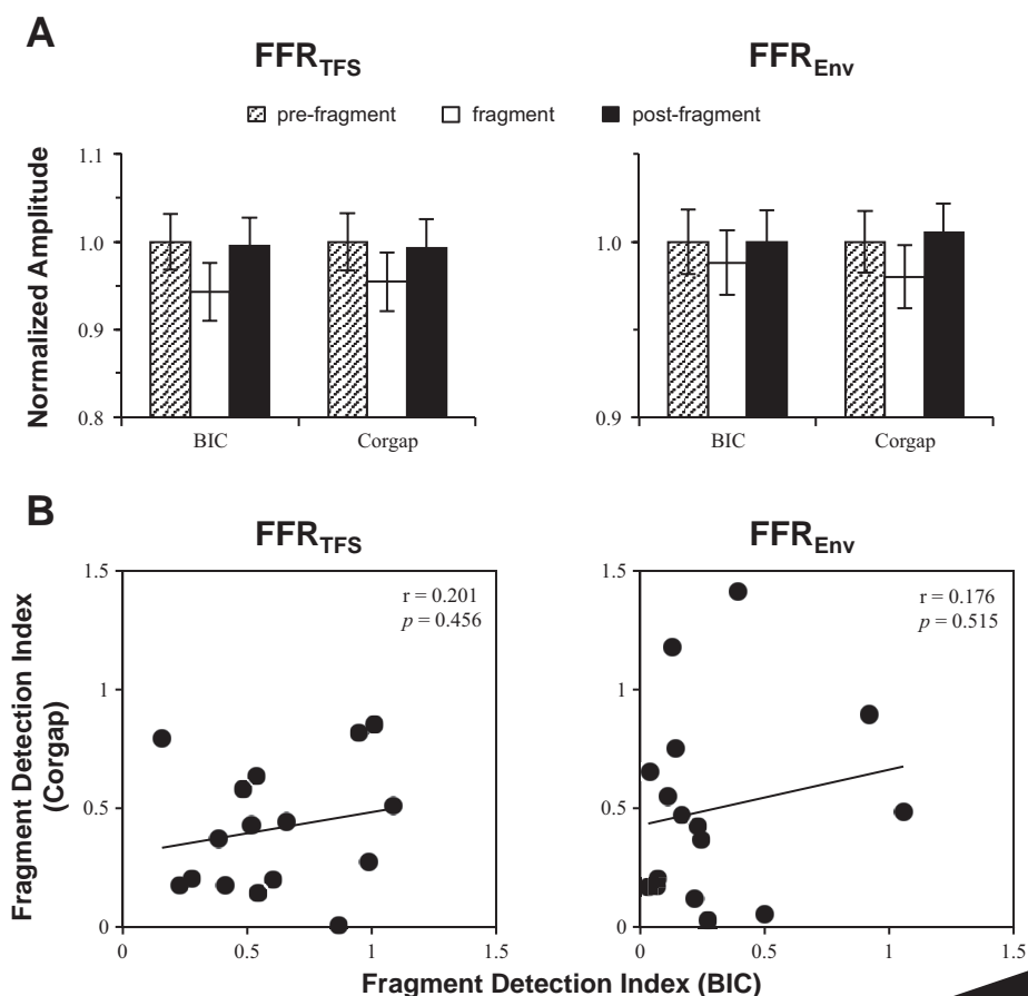
Fig. 3. A: comparisons in normalized FFR amplitude across stimulation conditions for the FFR_{TFS} (left) and the FFR_{Env} (right). Fragment period, 350–550 ms after sound onset; prefragment period, 100–300 ms after sound onset; postfragment period, 600–800 ms after sound onset. Error bars: SE. B: examinations of the correlation in the neural fragment detection index (FDI) between the BIC-stimulation condition and the Corgap-stimulation condition for the FFR_{TFS} (left) and the FFR_{Env} (right).
